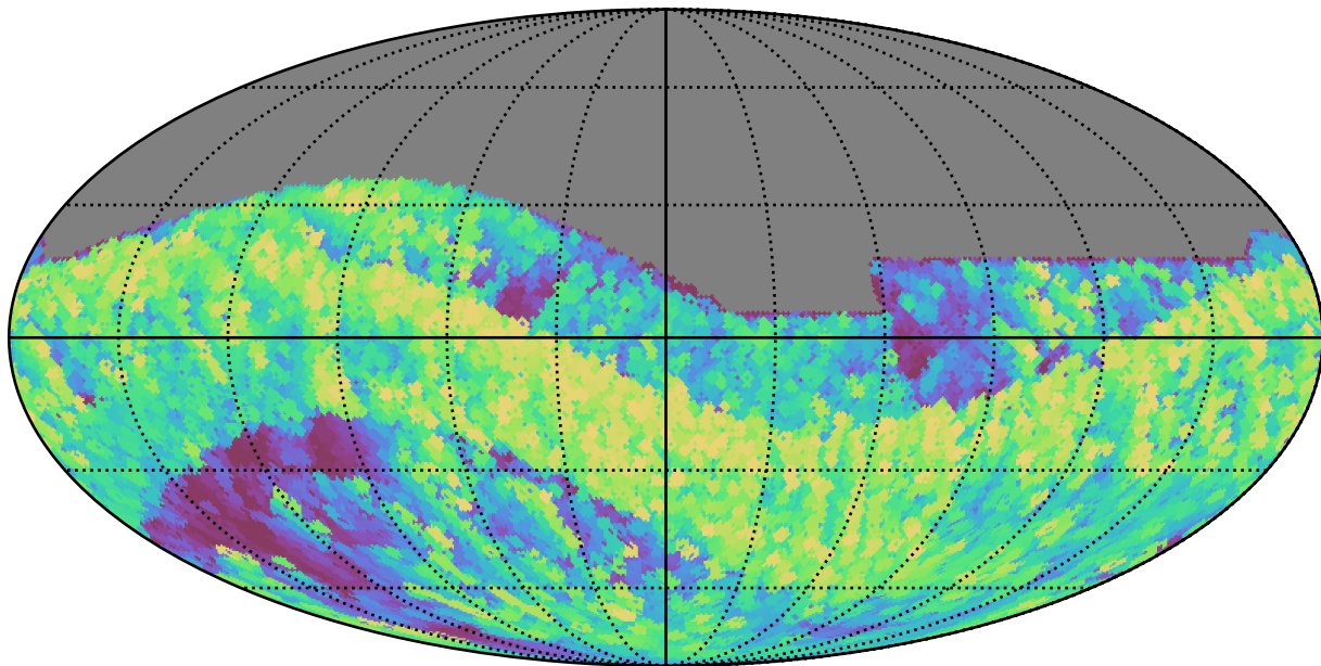
mw_roll_all_v3.3_10yrs All sky i band: Max airmass
