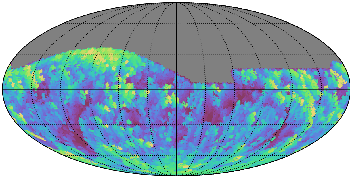
mw_roll_all_v3.3_10yrs All sky g band: Max airmass
