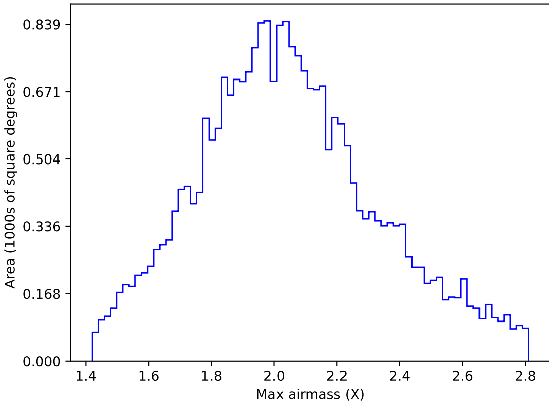
mw_roll_all_v3.3_10yrs All sky g band: Max airmass
