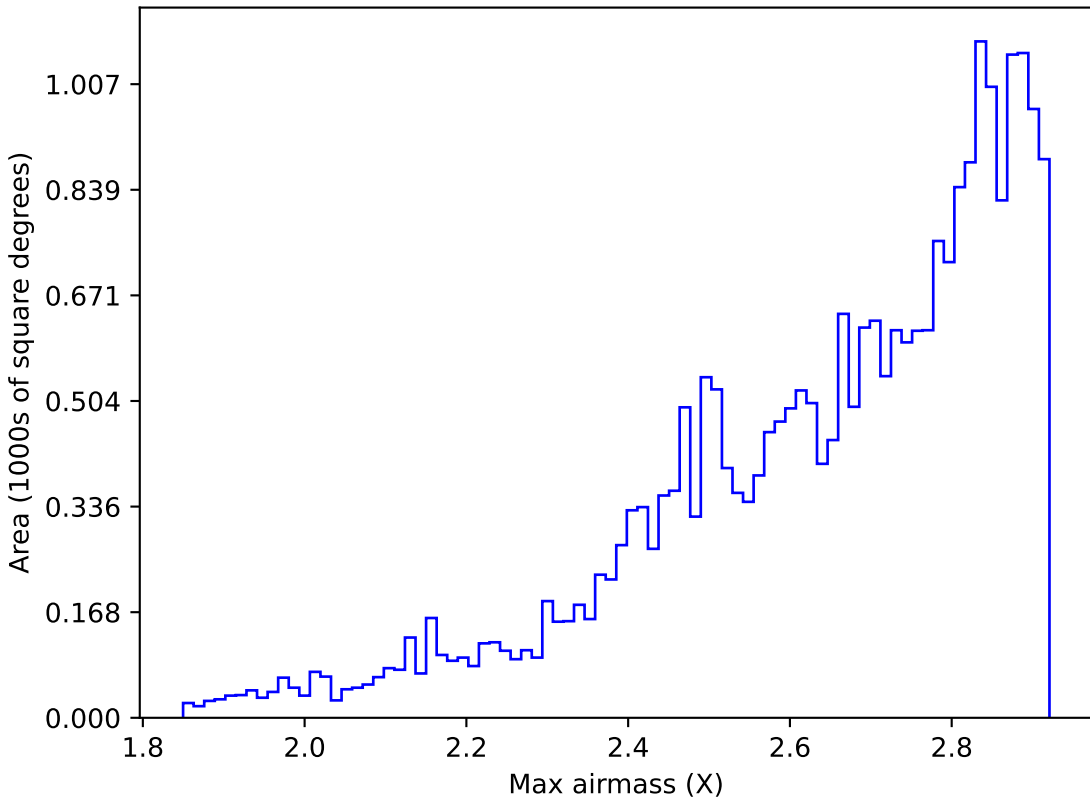
mw_roll_all_v3.3_10yrs All sky all bands: Max airmass
