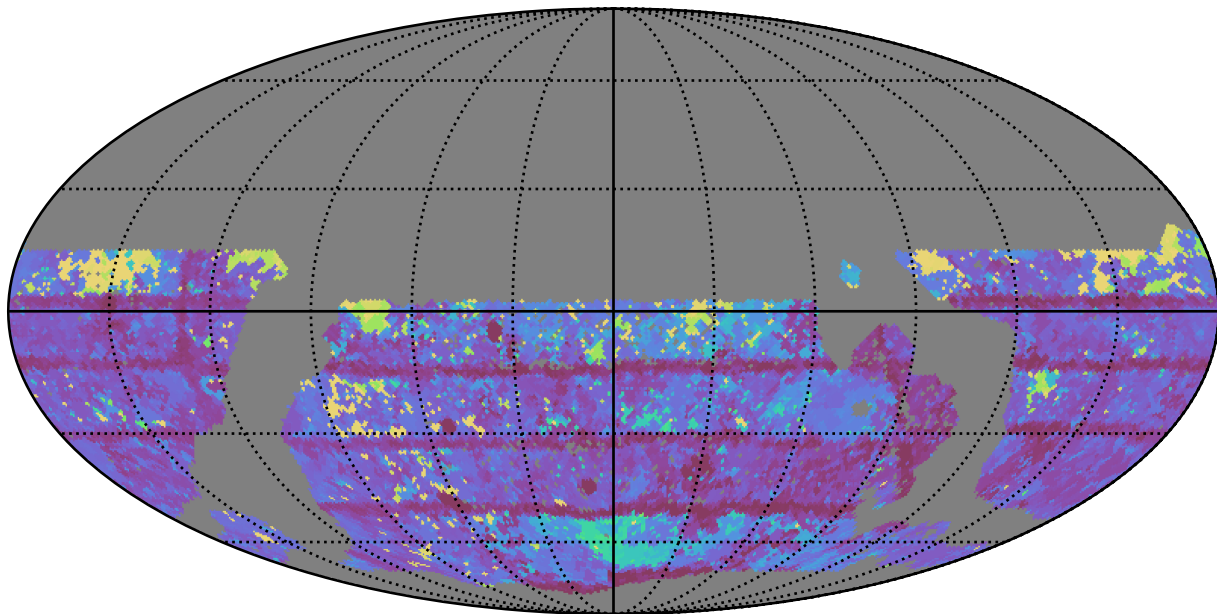
mw_roll_all_v3.3_10yrs WFD z band: Max Inter-Night Gap
