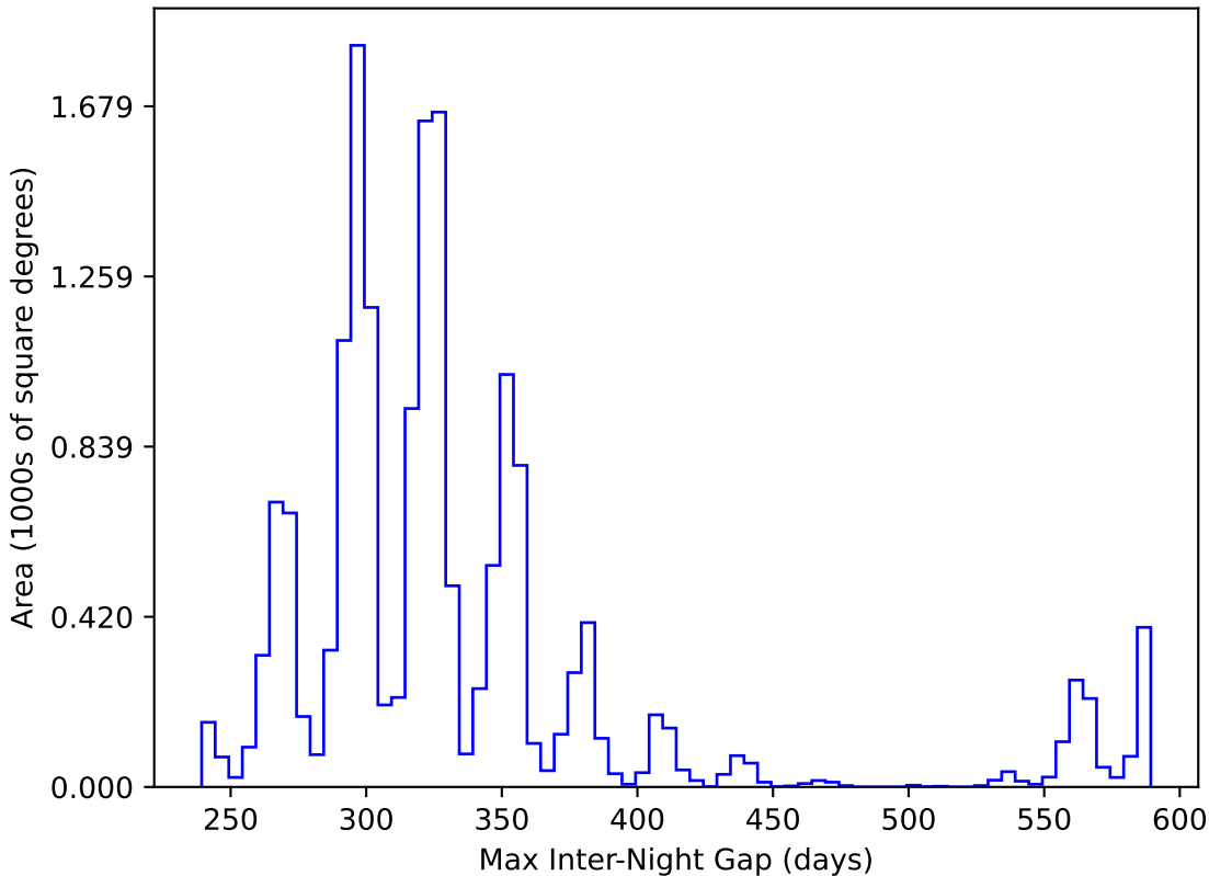
mw_roll_all_v3.3_10yrs WFD y band: Max Inter-Night Gap
