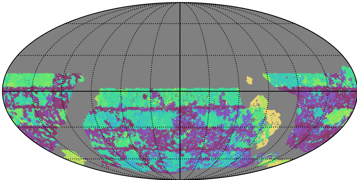
mw_roll_all_v3.3_10yrs WFD u band: Max Inter-Night Gap
