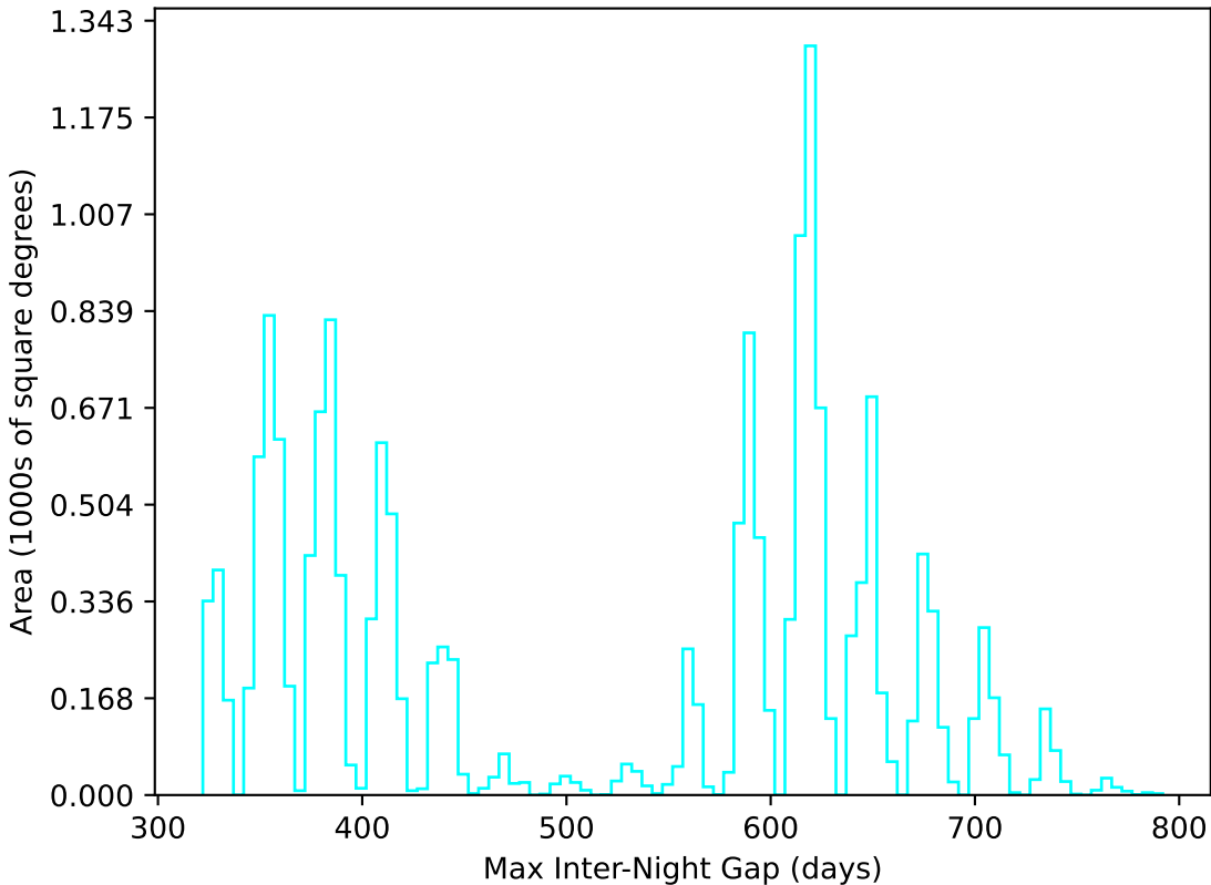
mw_roll_all_v3.3_10yrs WFD u band: Max Inter-Night Gap
