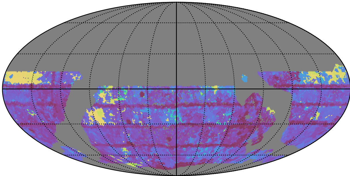
mw_roll_all_v3.3_10yrs WFD r band: Max Inter-Night Gap
