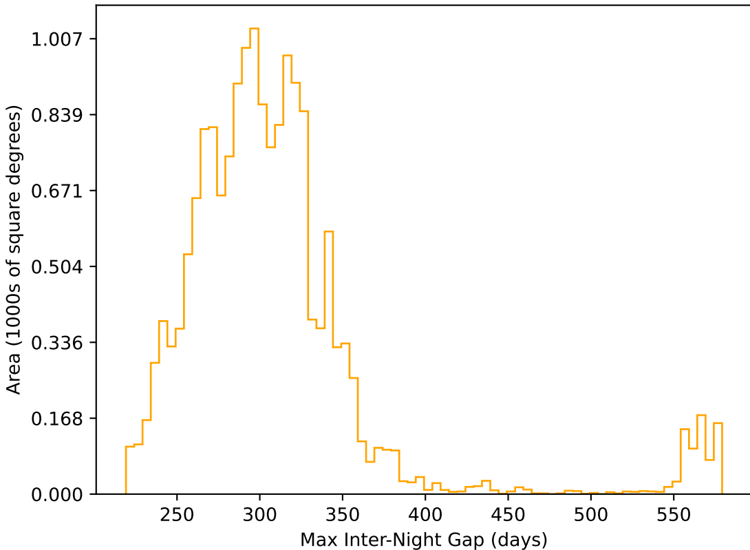
mw_roll_all_v3.3_10yrs WFD r band: Max Inter-Night Gap
