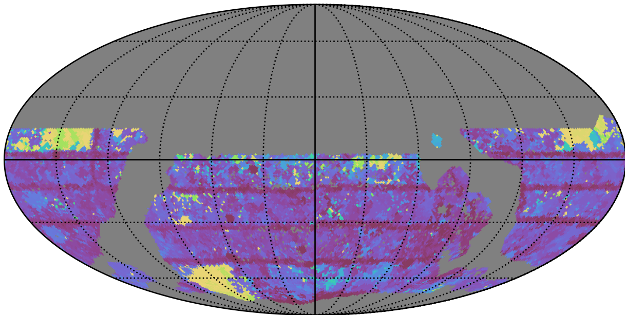
mw_roll_all_v3.3_10yrs WFD i band: Max Inter-Night Gap
