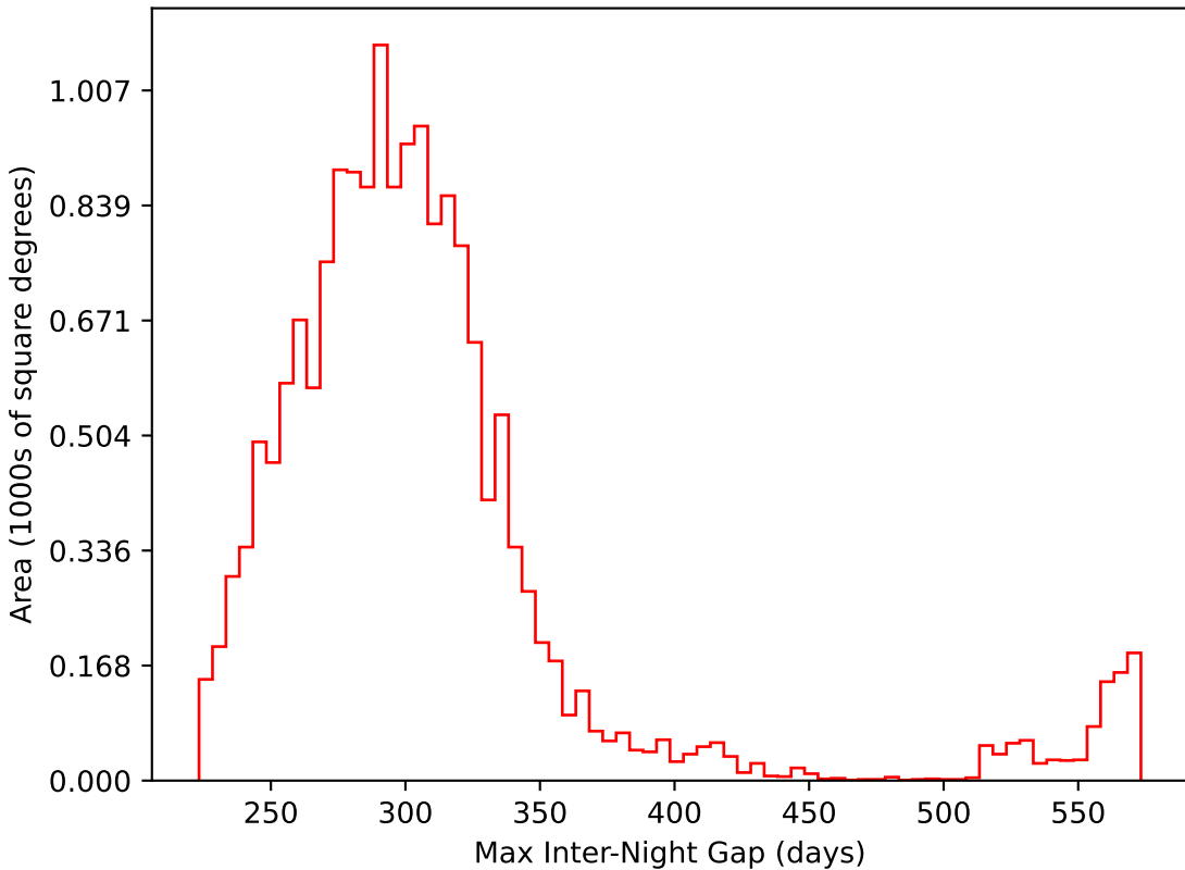
mw_roll_all_v3.3_10yrs WFD i band: Max Inter-Night Gap
