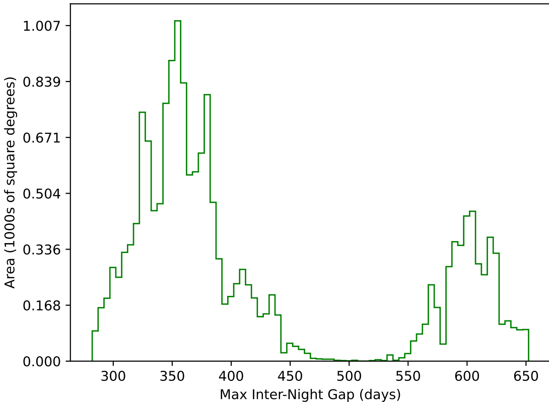
mw_roll_all_v3.3_10yrs WFD g band: Max Inter-Night Gap
