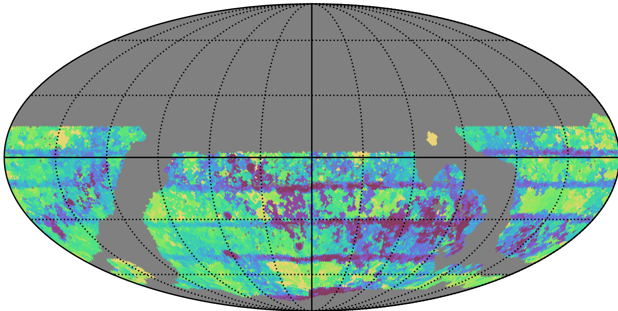
mw_roll_all_v3.3_10yrs WFD all bands: Max Inter-Night Gap
