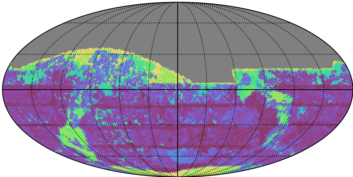
mw_roll_all_v3.3_10yrs All sky z band: Max Inter-Night Gap
