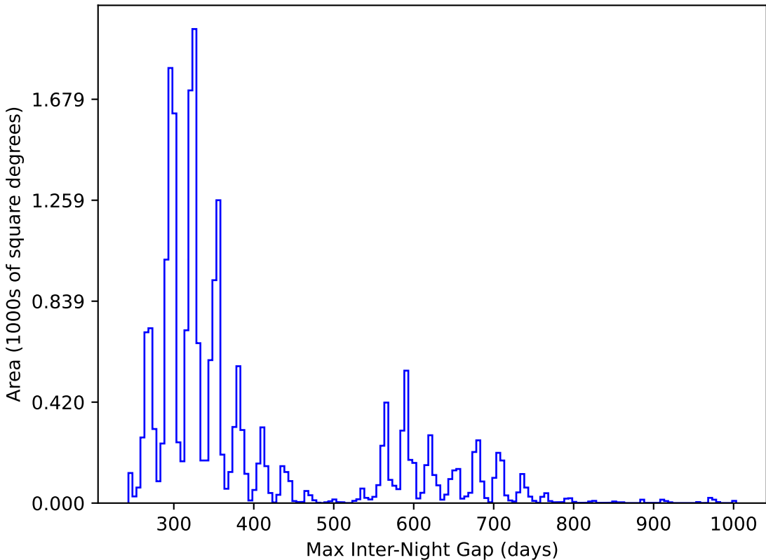
mw_roll_all_v3.3_10yrs All sky y band: Max Inter-Night Gap
