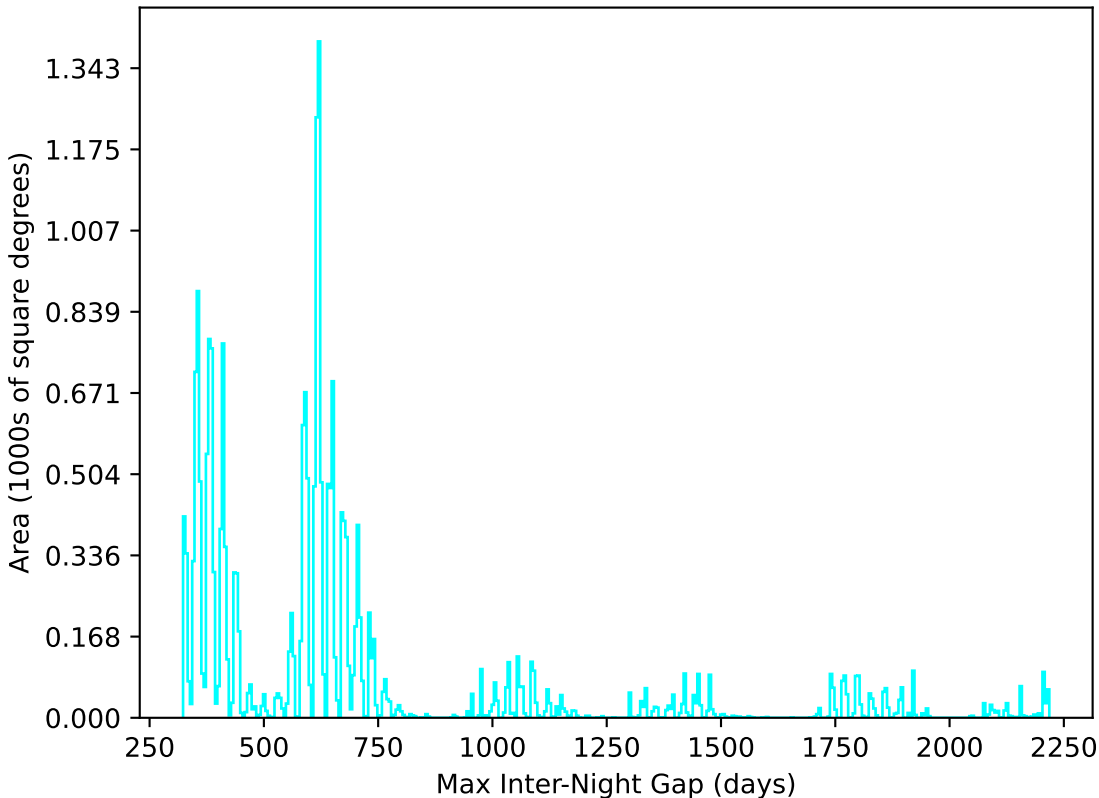
mw_roll_all_v3.3_10yrs All sky u band: Max Inter-Night Gap
