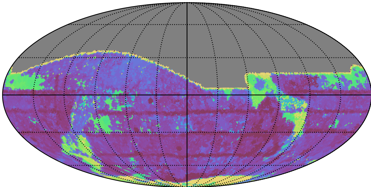
mw_roll_all_v3.3_10yrs All sky r band: Max Inter-Night Gap
