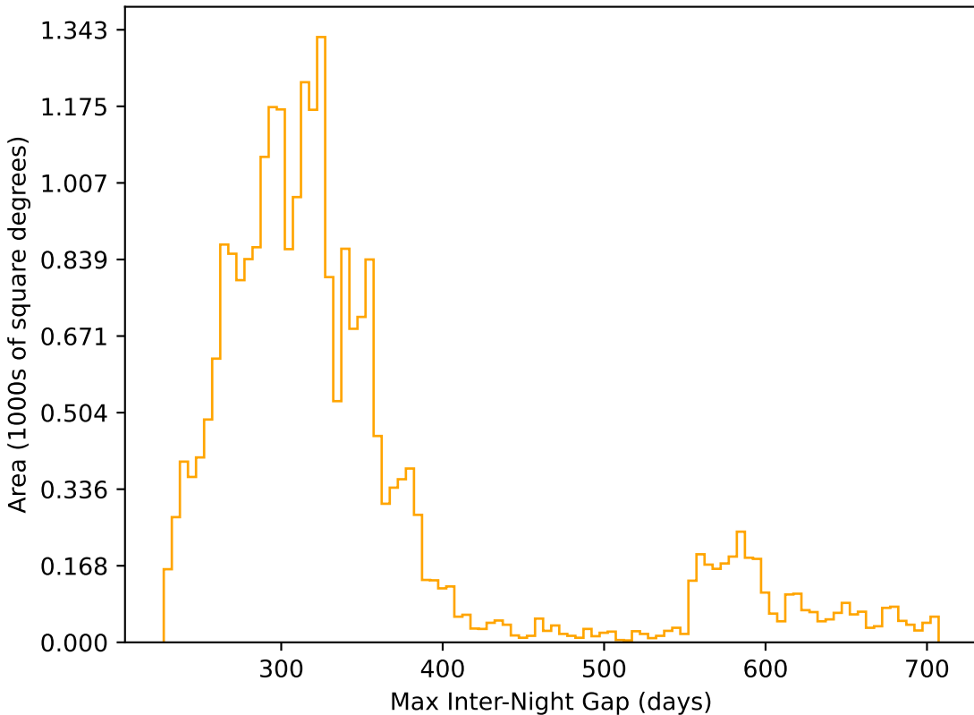
mw_roll_all_v3.3_10yrs All sky r band: Max Inter-Night Gap
