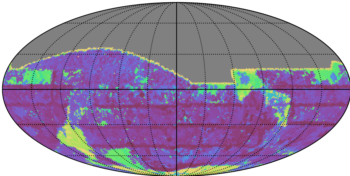
mw_roll_all_v3.3_10yrs All sky i band: Max Inter-Night Gap
