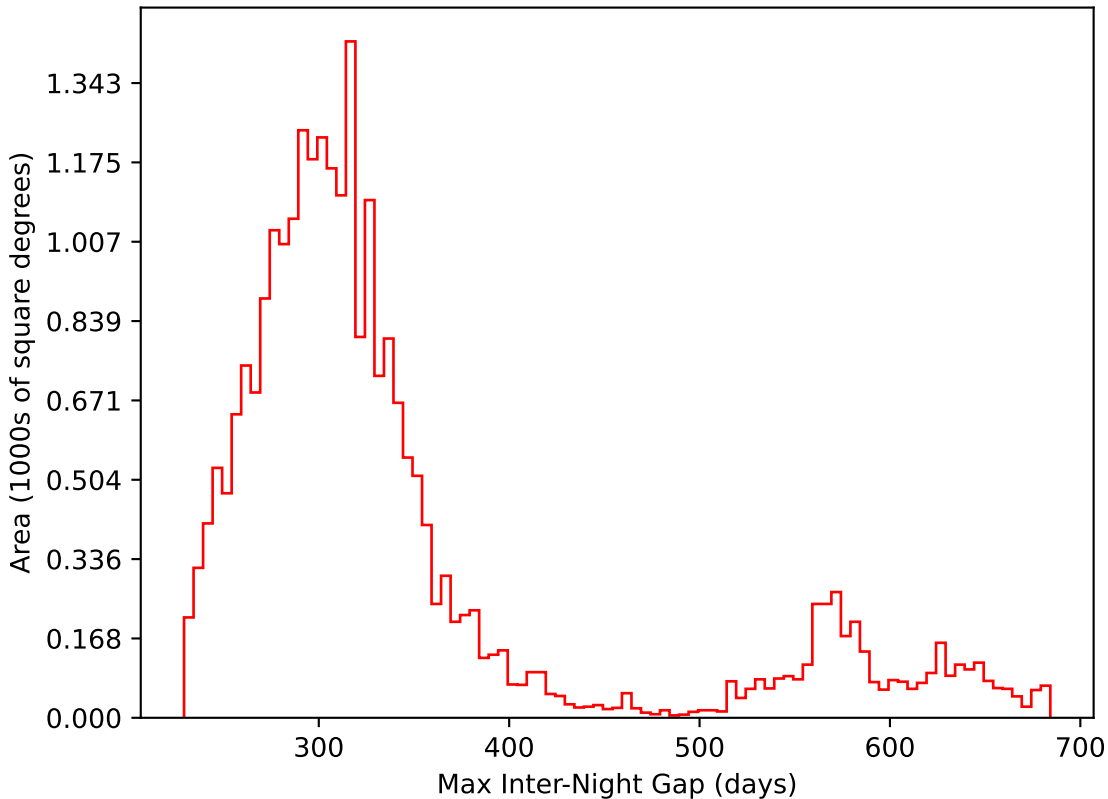
mw_roll_all_v3.3_10yrs All sky i band: Max Inter-Night Gap
