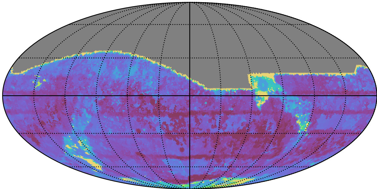
mw_roll_all_v3.3_10yrs All sky all bands: Max Inter-Night Gap
