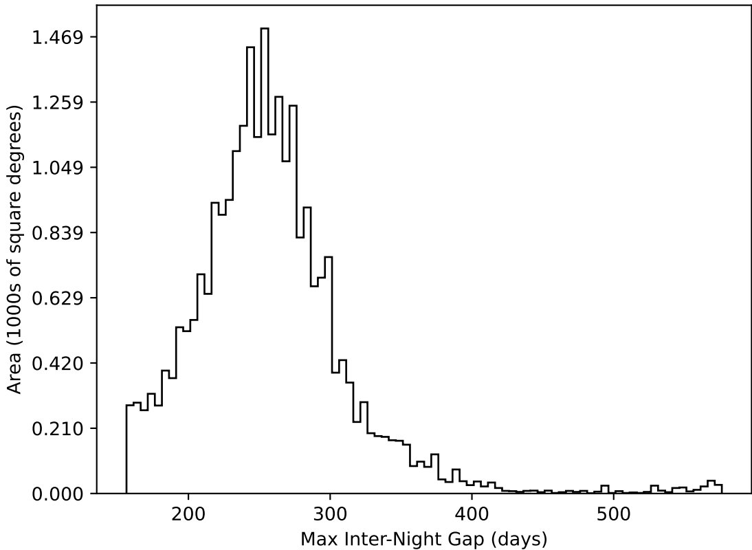
mw_roll_all_v3.3_10yrs All sky all bands: Max Inter-Night Gap
