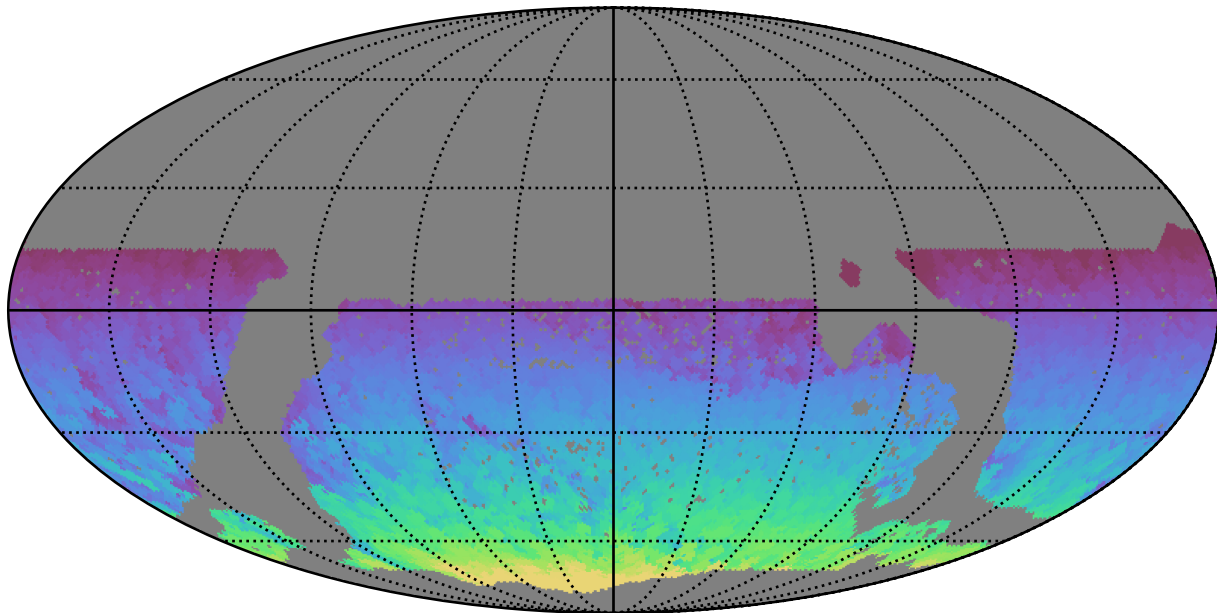
mw_roll_all_v3.3_10yrs WFD all bands: Max HA
