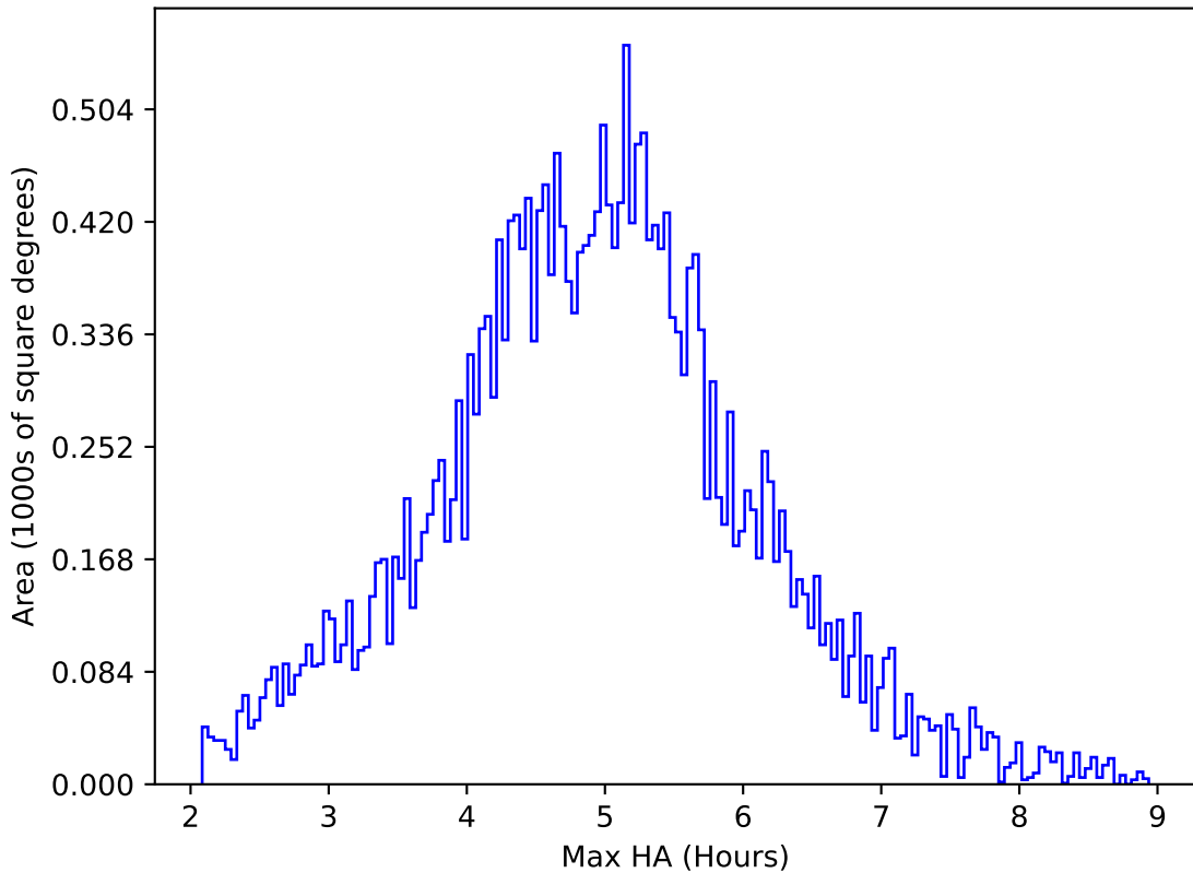
mw_roll_all_v3.3_10yrs All sky all bands: Max HA
