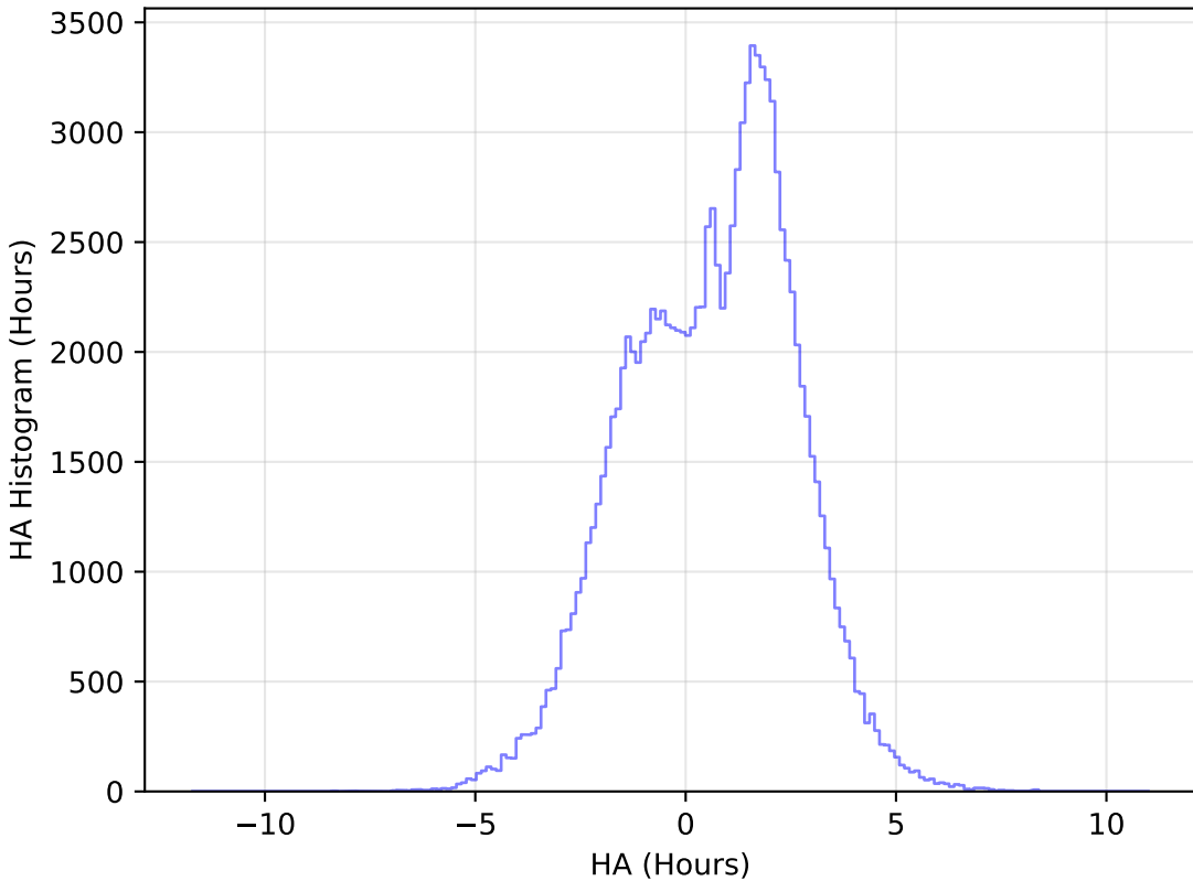
mw_roll_all_v3.3_10yrs WFD u band: HA Histogram
