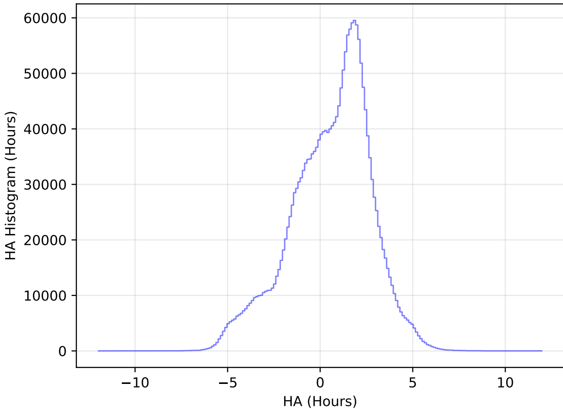
mw_roll_all_v3.3_10yrs WFD all bands: HA Histogram
