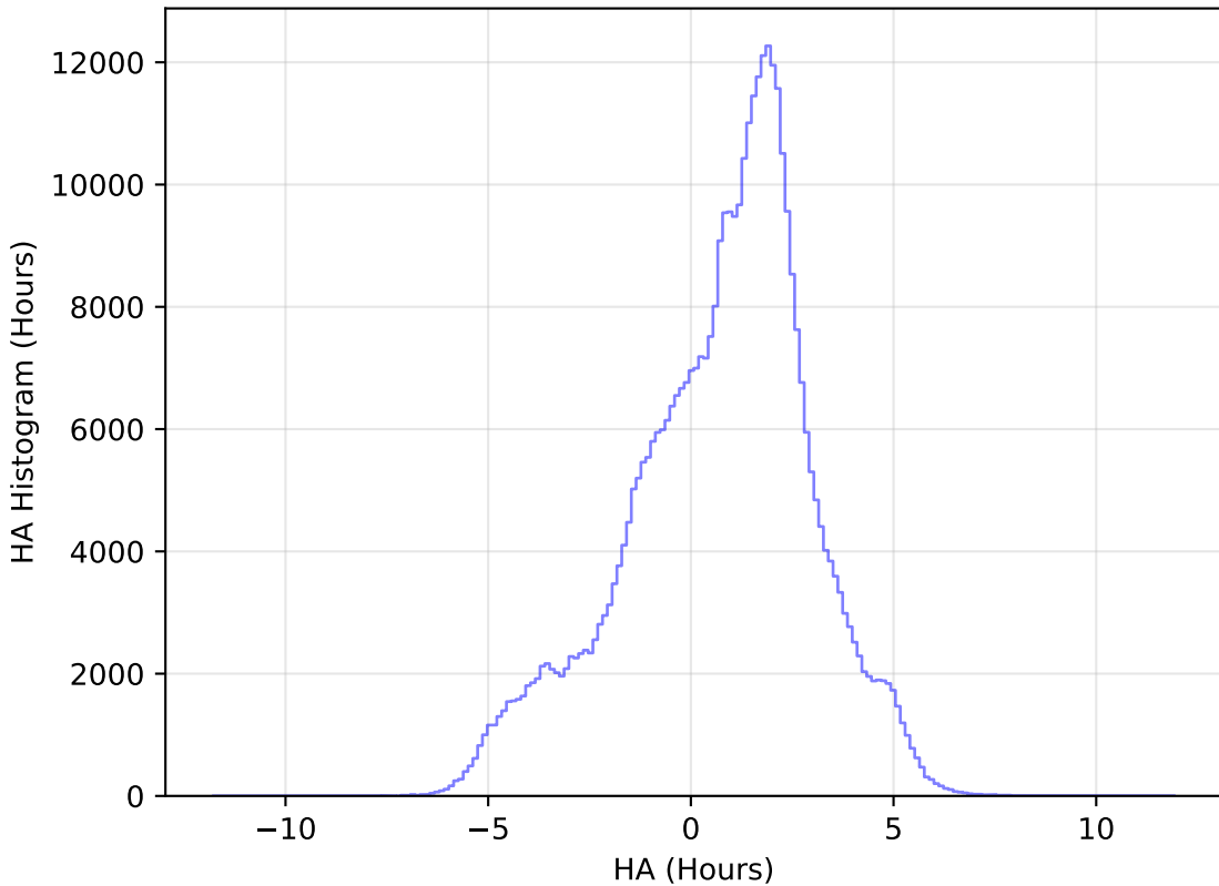
mw_roll_all_v3.3_10yrs All sky z band: HA Histogram
