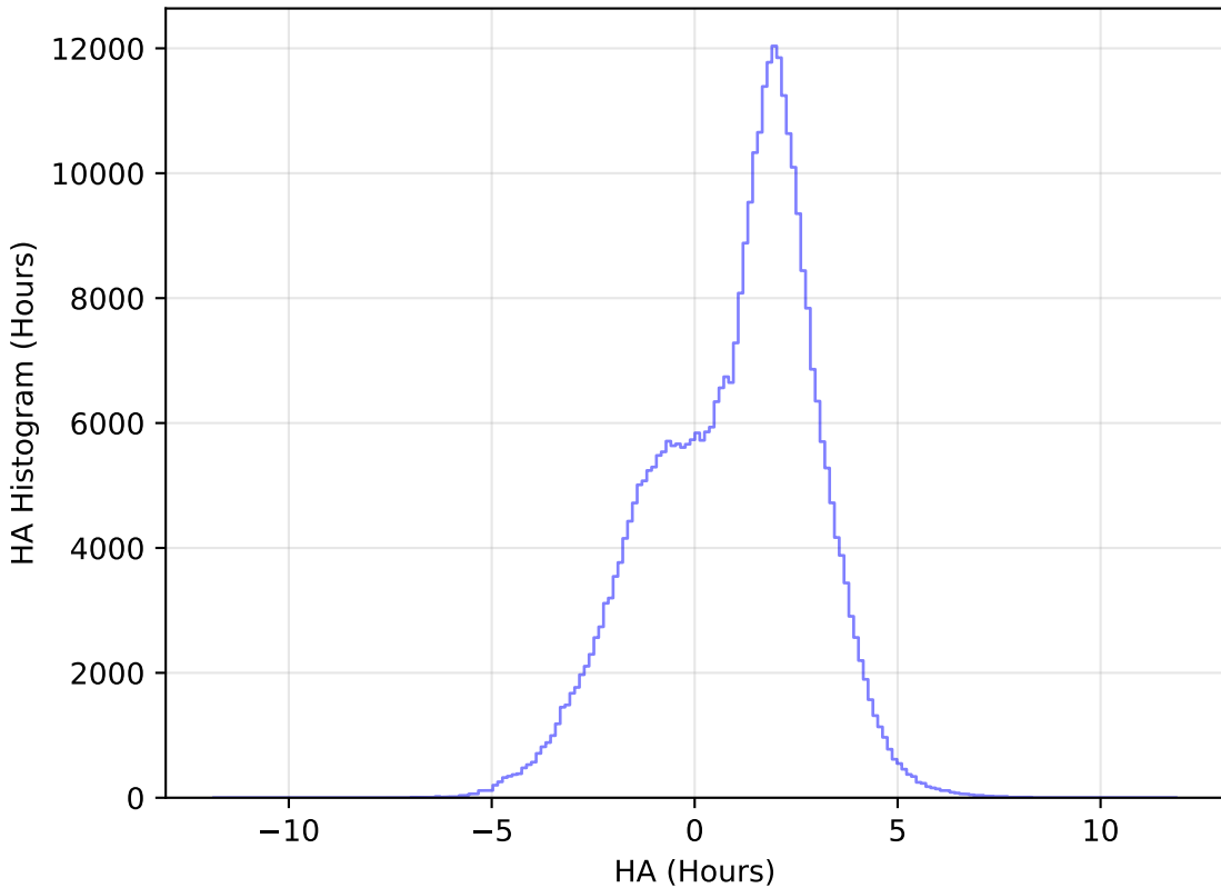
mw_roll_all_v3.3_10yrs All sky y band: HA Histogram
