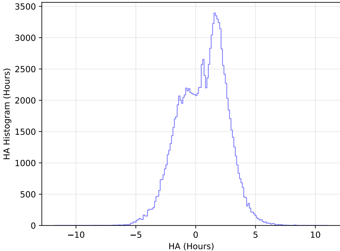
mw_roll_all_v3.3_10yrs All sky u band: HA Histogram
