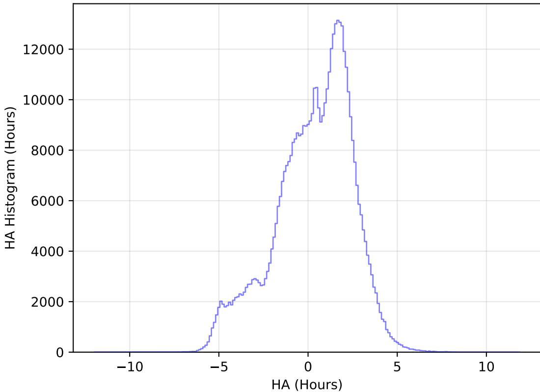
mw_roll_all_v3.3_10yrs All sky r band: HA Histogram
