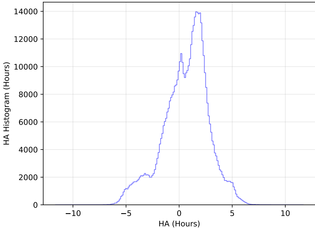
mw_roll_all_v3.3_10yrs All sky i band: HA Histogram
