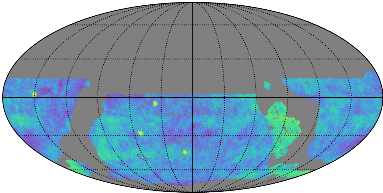
mw_roll_all_v3.3_10yrs gri WFD: Fraction of visits in pairs (20-90 min)
