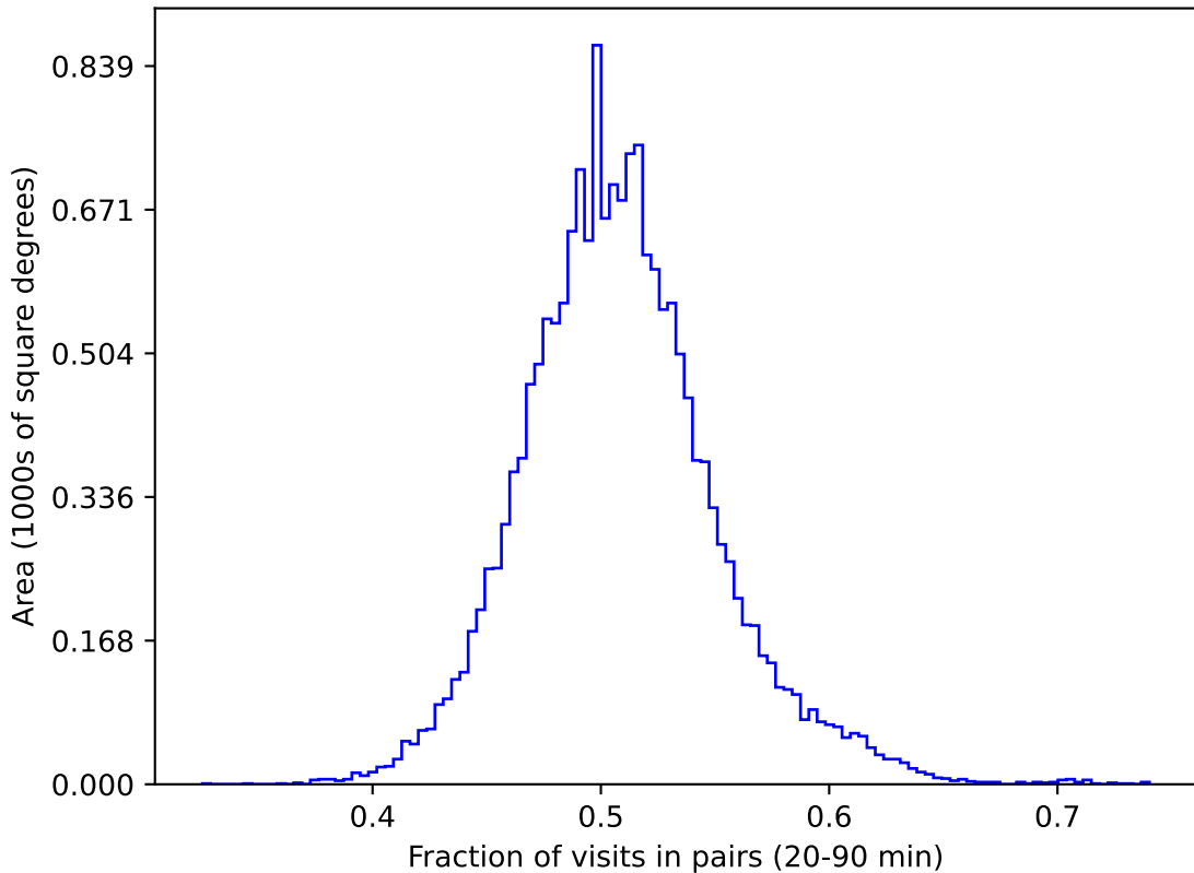
mw_roll_all_v3.3_10yrs gri WFD: Fraction of visits in pairs (20-90 min)
