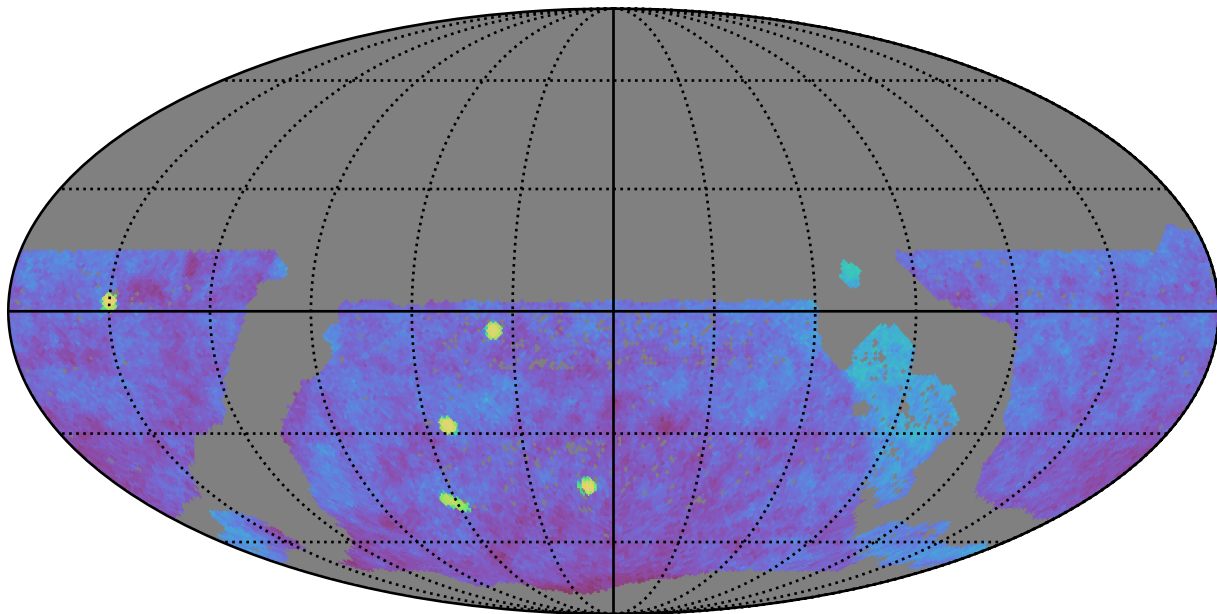
mw_roll_all_v3.3_10yrs gri WFD: Fraction of visits in pairs (10-60 min)
