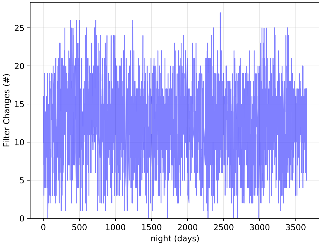
mw_roll_all_v3.3_10yrs Per Night: Filter Changes
