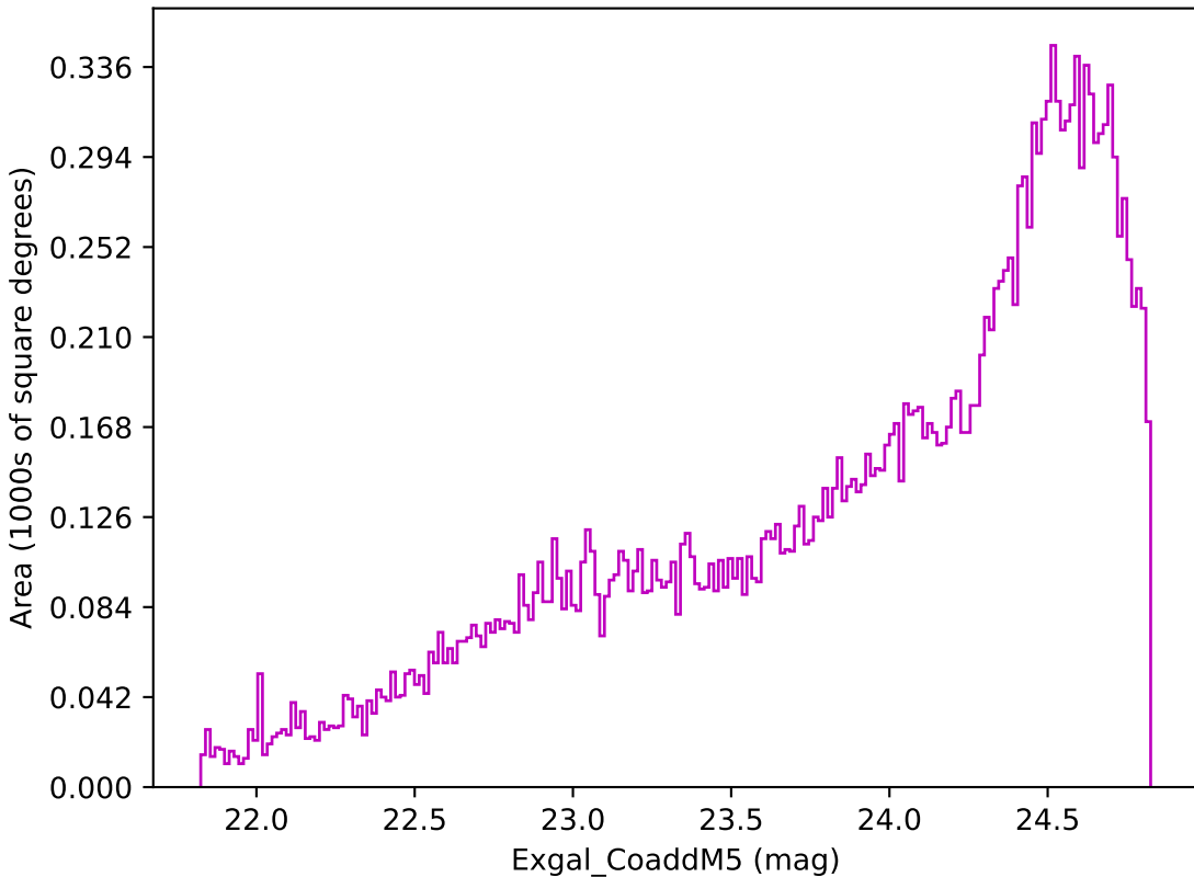
mw_roll_all_v3.3_10yrs Yr 3-4 z band: Exgal_CoaddM5
