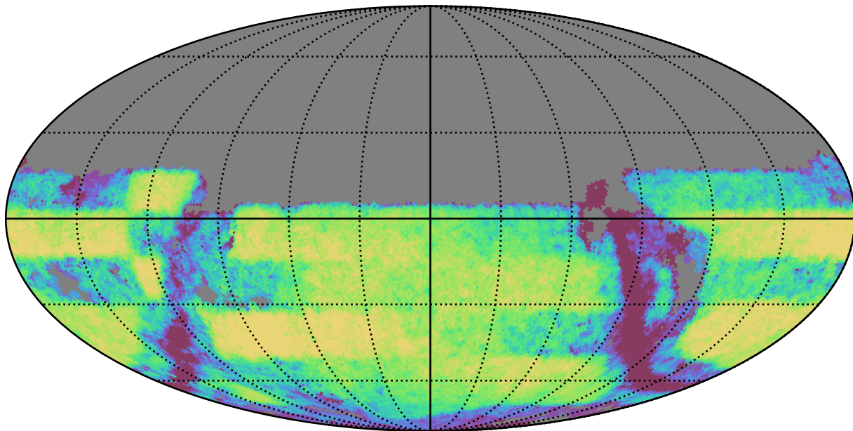
mw_roll_all_v3.3_10yrs Yr 3-4 y band: Exgal_CoaddM5
