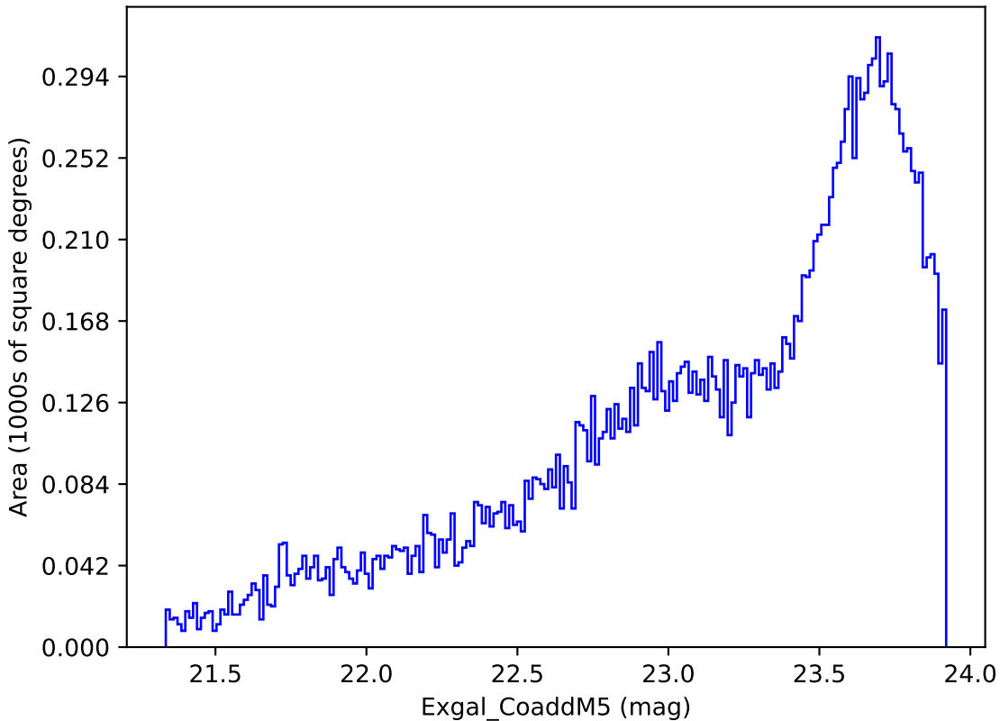
mw_roll_all_v3.3_10yrs Yr 3-4 y band: Exgal_CoaddM5
