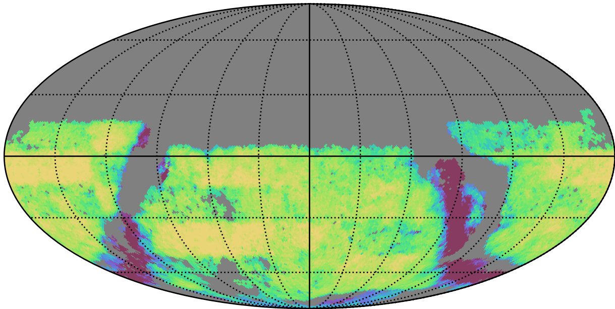
mw_roll_all_v3.3_10yrs Yr 3-4 u band: Exgal_CoaddM5
