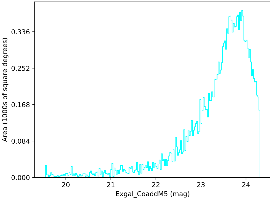
mw_roll_all_v3.3_10yrs Yr 3-4 u band: Exgal_CoaddM5
