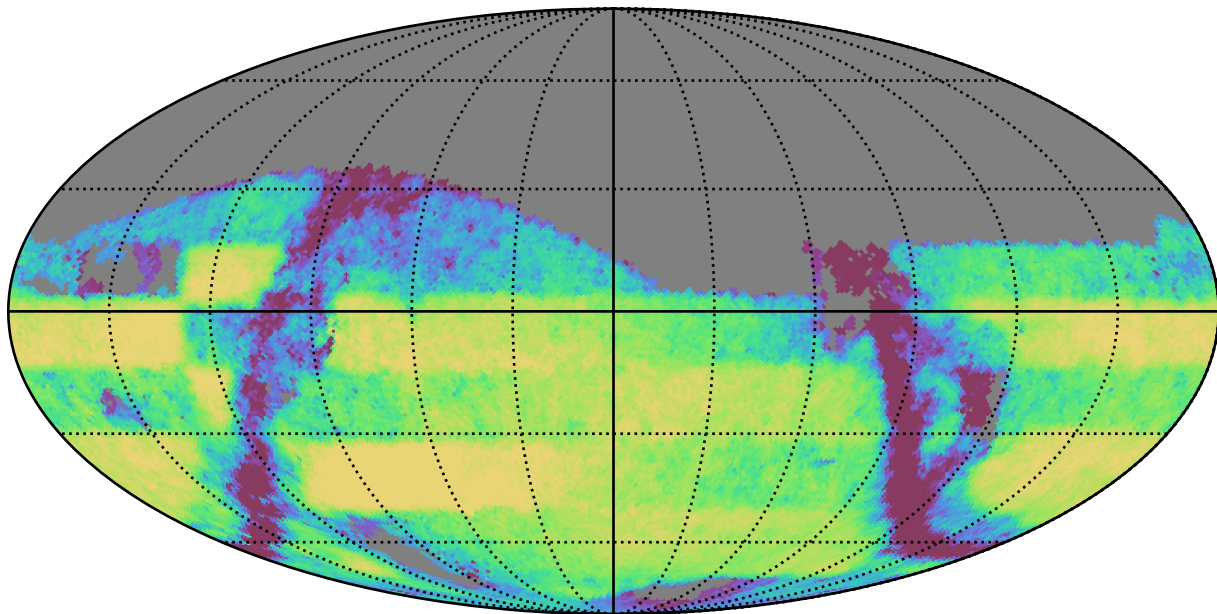
mw_roll_all_v3.3_10yrs Yr 3-4 i band: Exgal_CoaddM5
