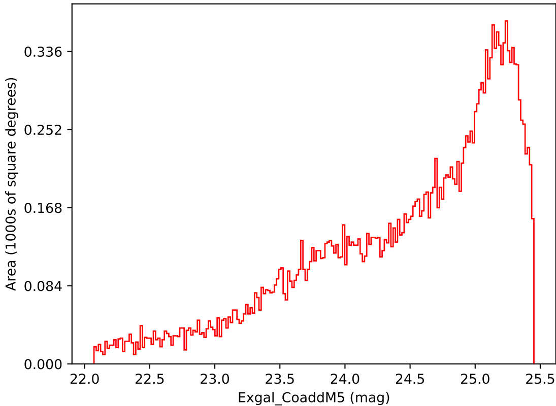
mw_roll_all_v3.3_10yrs Yr 3-4 i band: Exgal_CoaddM5
