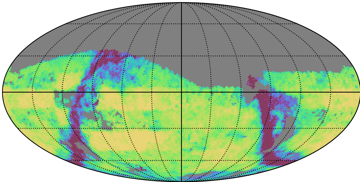
mw_roll_all_v3.3_10yrs Yr 3-4 g band: Exgal_CoaddM5
