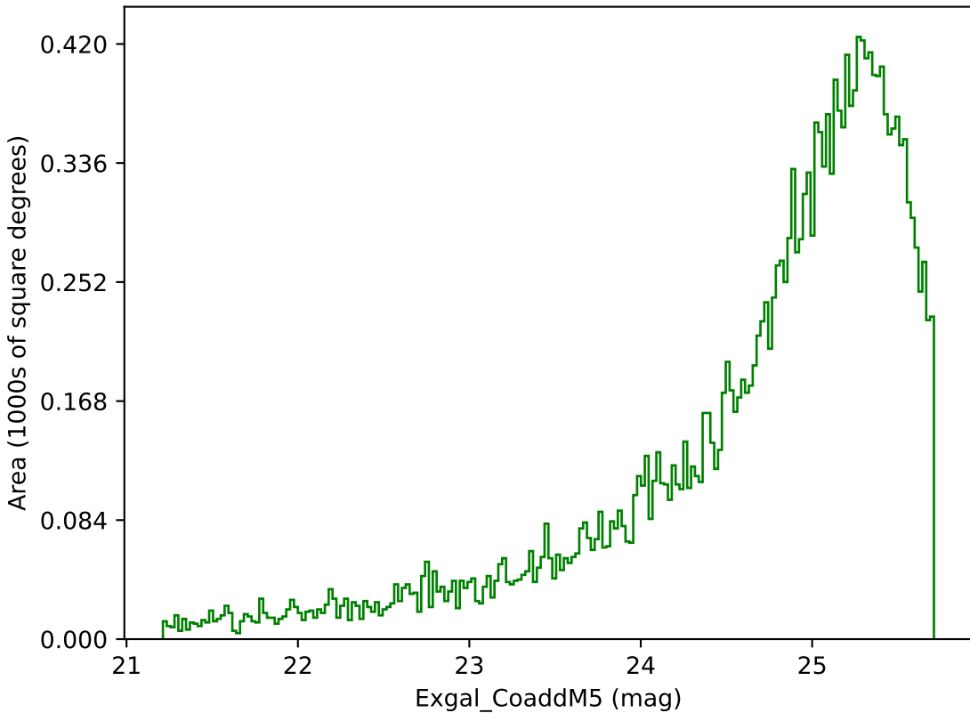
mw_roll_all_v3.3_10yrs Yr 3-4 g band: Exgal_CoaddM5
