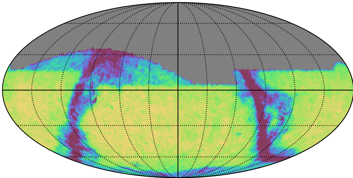
mw_roll_all_v3.3_10yrs Yr 1 z band: Exgal_CoaddM5
