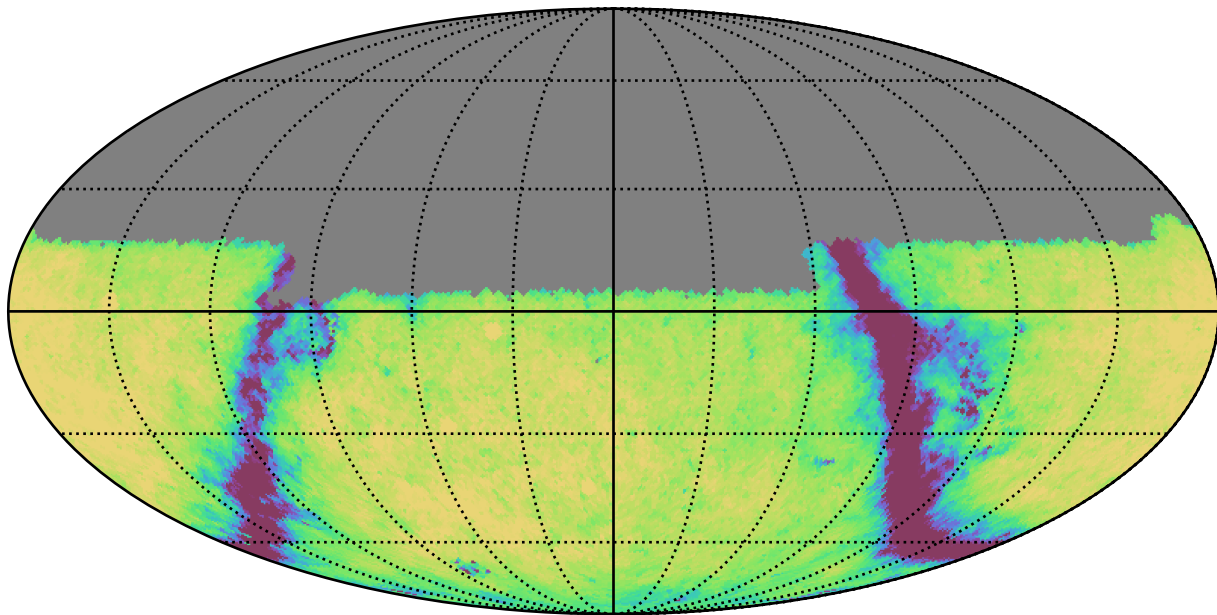
mw_roll_all_v3.3_10yrs Yr 1 u band: Exgal_CoaddM5
