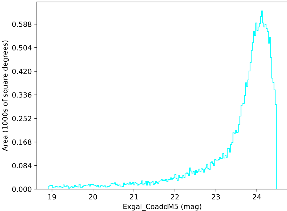
mw_roll_all_v3.3_10yrs Yr 1 u band: Exgal_CoaddM5
