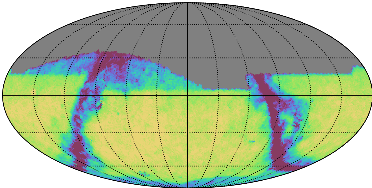
mw_roll_all_v3.3_10yrs Yr 1 i band: Exgal_CoaddM5
