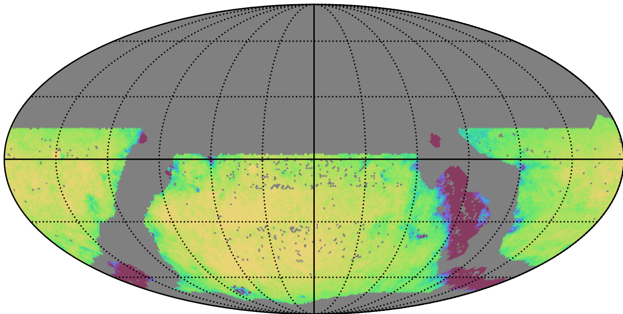
mw_roll_all_v3.3_10yrs WFD u band: Exgal_CoaddM5
